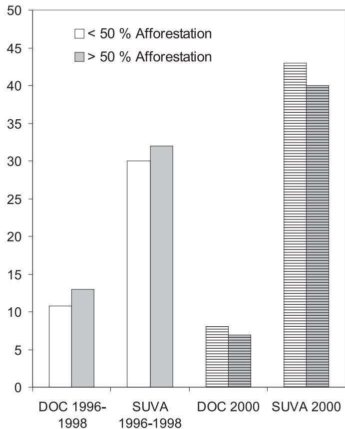
Fig. 5. Changes of DOC concentration ( \text{mg dm}^{-3} ) and SUVA ( \text{Abs}_{260} \text{ g C}^{-1} \text{ dm}^{-3} ) (formula 1) in two groups of catchment afforestation in wet/normal October (1996–1998) and during drought (October 2000).
